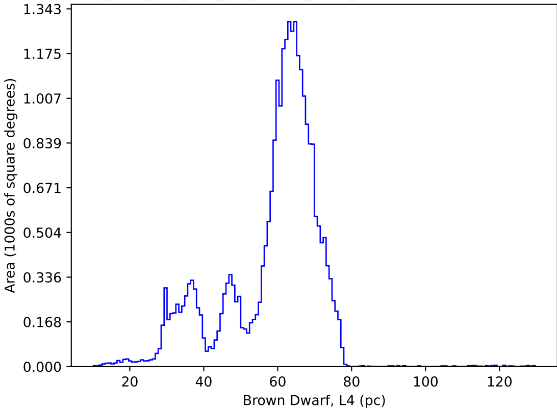
too_elab_2yr_r64_d3_ugrizy_v3.4_10yrs : Brown Dwarf, L4
