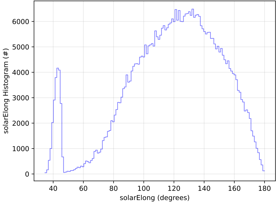
too_elab_2yr_r64_d3_ugrizy_v3.4_10yrs WFD z band: solarElong Histogram
