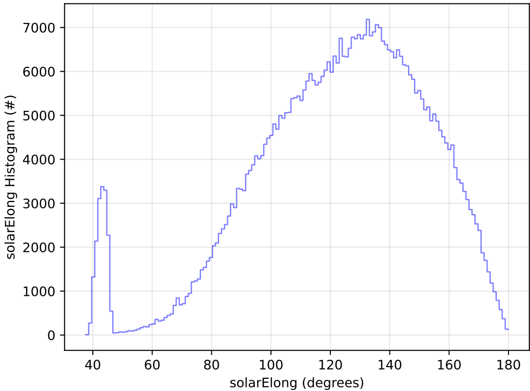
too_elab_2yr_r64_d3_ugrizy_v3.4_10yrs WFD r band: solarElong Histogram
