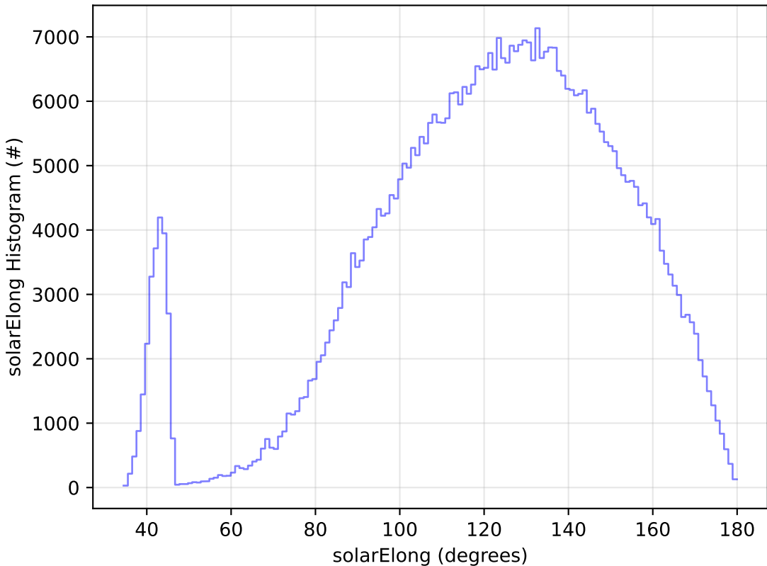
too_elab_2yr_r64_d3_ugrizy_v3.4_10yrs WFD i band: solarElong Histogram
