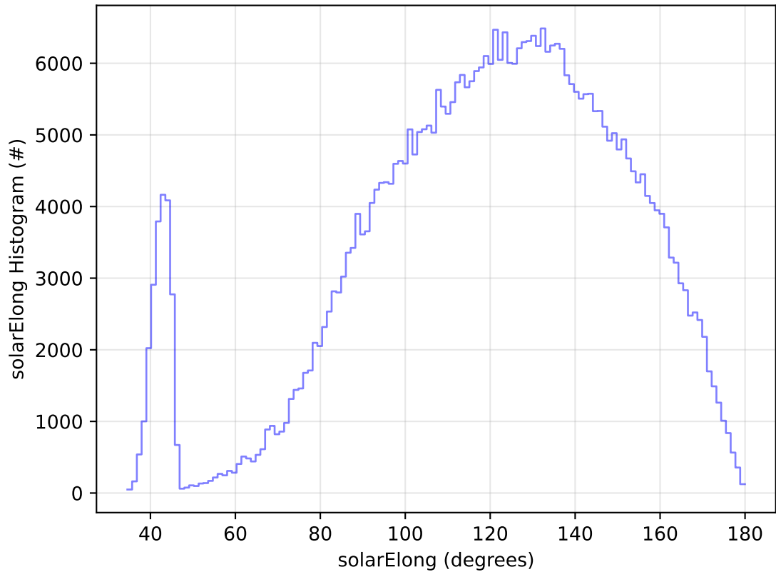
too_elab_2yr_r64_d3_ugrizy_v3.4_10yrs All sky z band: solarElong Histogram
