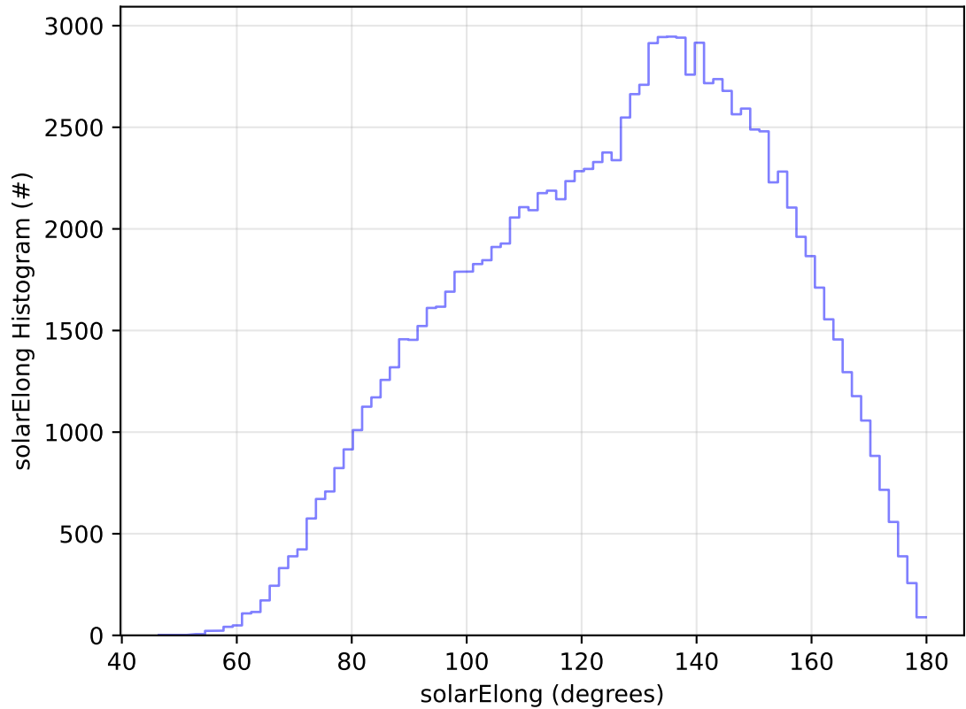
too_elab_2yr_r64_d3_ugrizy_v3.4_10yrs All sky u band: solarElong Histogram
