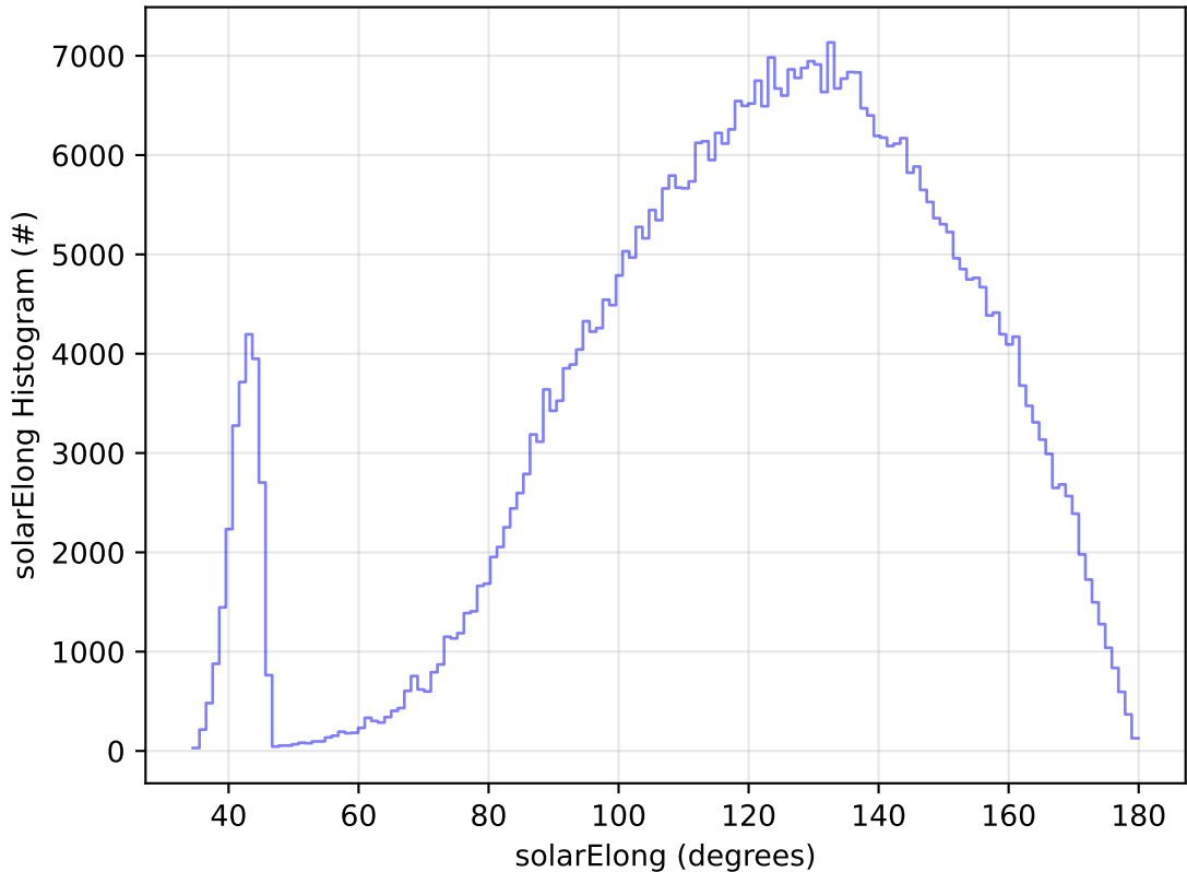
too_elab_2yr_r64_d3_ugrizy_v3.4_10yrs All sky i band: solarElong Histogram
