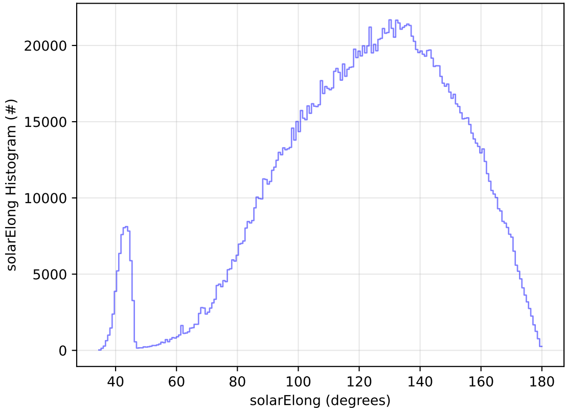
too_elab_2yr_r64_d3_ugrizy_v3.4_10yrs All sky all bands: solarElong Histogram
