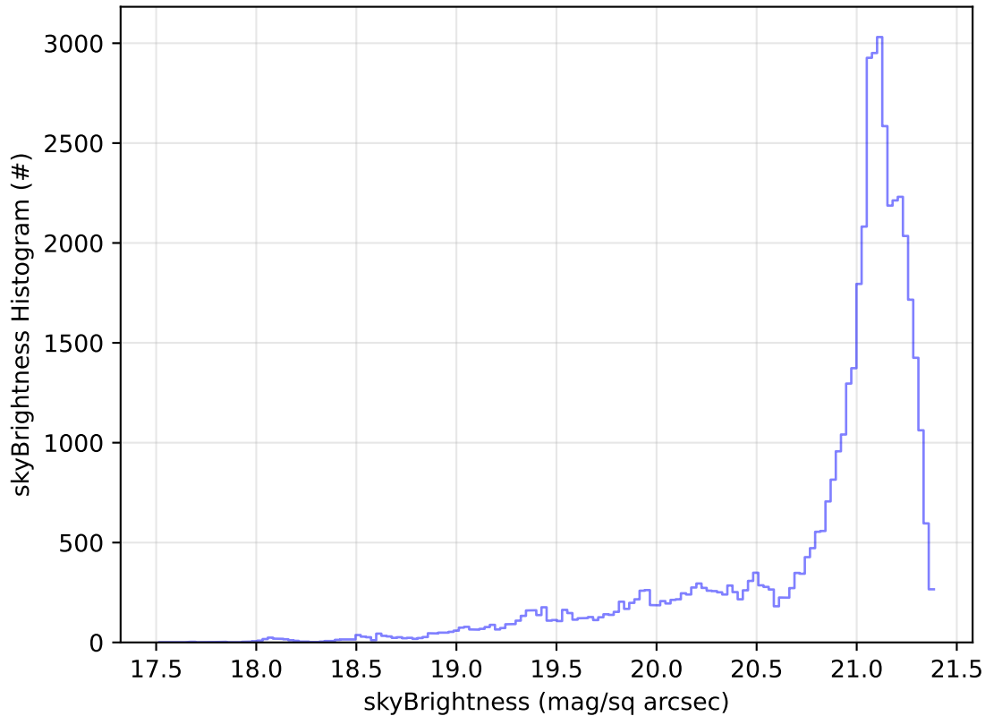
too_elab_2yr_r64_d3_ugrizy_v3.4_10yrs Yr 1 r band: skyBrightness Histogram
