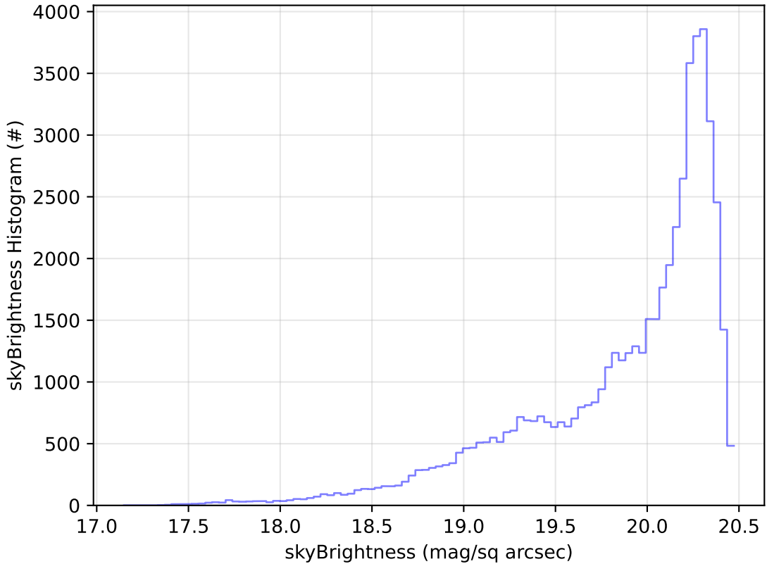
too_elab_2yr_r64_d3_ugrizy_v3.4_10yrs Yr 1 i band: skyBrightness Histogram
