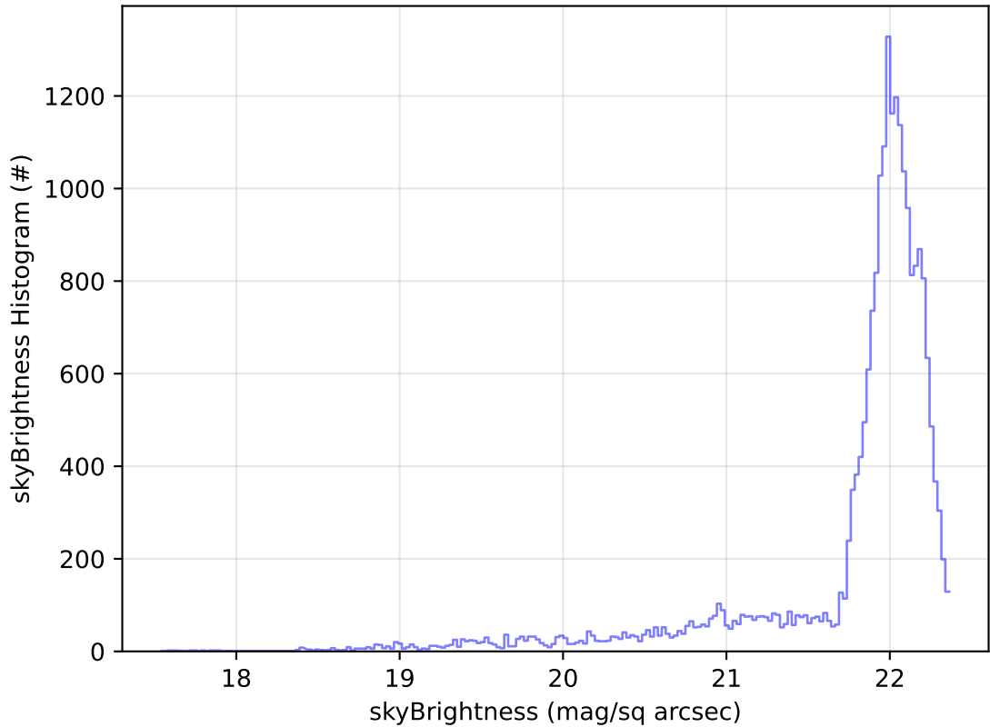
too_elab_2yr_r64_d3_ugrizy_v3.4_10yrs Yr 1 g band: skyBrightness Histogram
