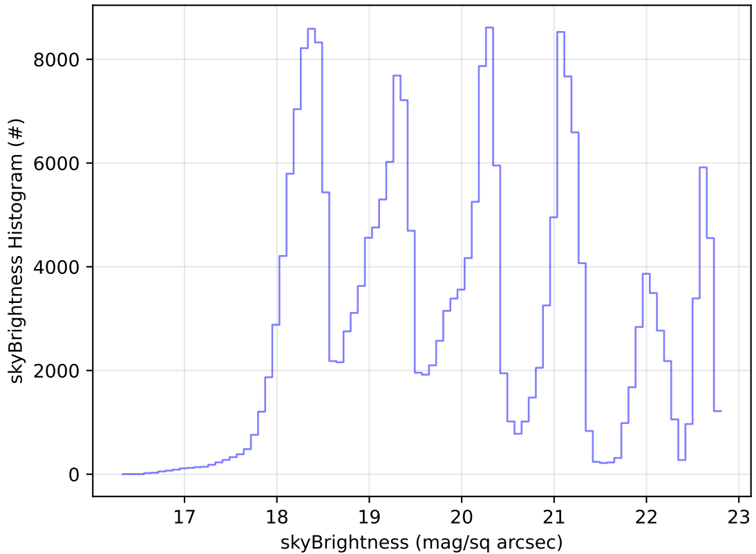
too_elab_2yr_r64_d3_ugrizy_v3.4_10yrs Yr 1 all bands: skyBrightness Histogram
