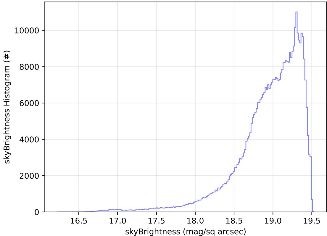
too_elab_2yr_r64_d3_ugrizy_v3.4_10yrs WFD z band: skyBrightness Histogram
