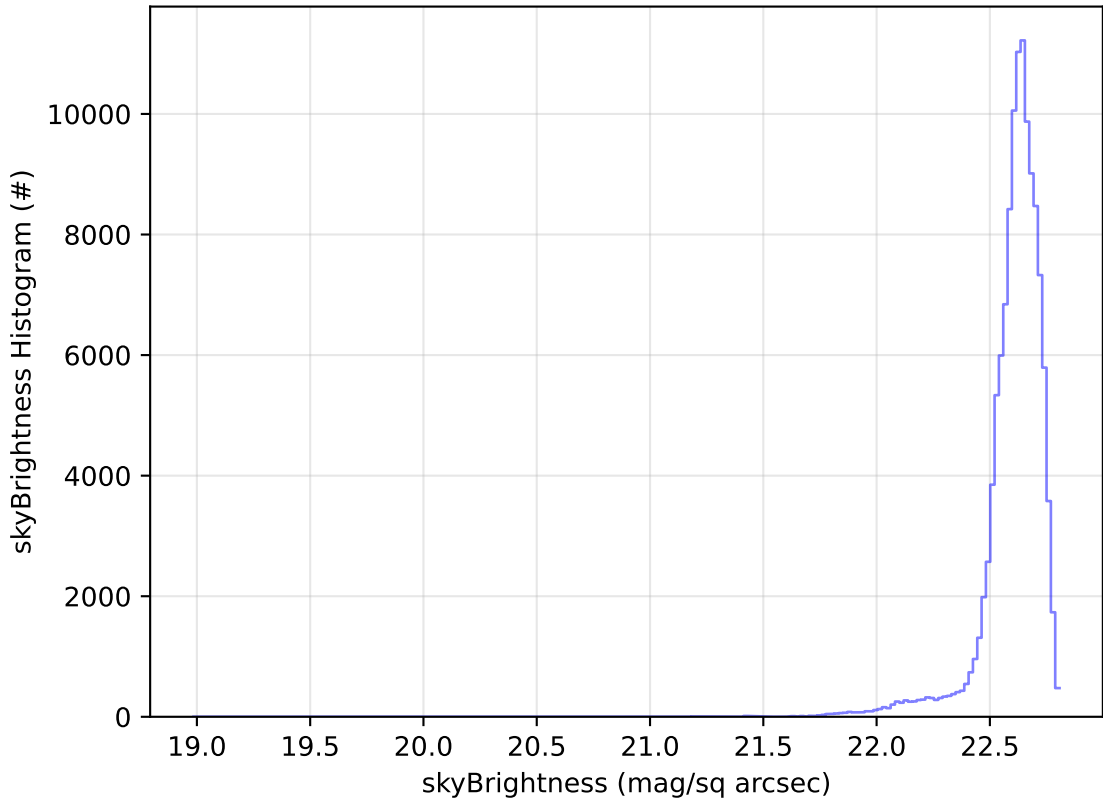
too_elab_2yr_r64_d3_ugrizy_v3.4_10yrs WFD u band: skyBrightness Histogram
