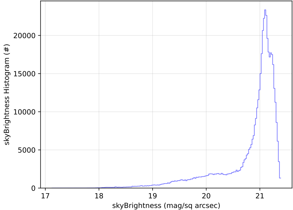
too_elab_2yr_r64_d3_ugrizy_v3.4_10yrs WFD r band: skyBrightness Histogram
