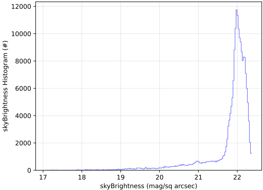
too_elab_2yr_r64_d3_ugrizy_v3.4_10yrs WFD g band: skyBrightness Histogram
