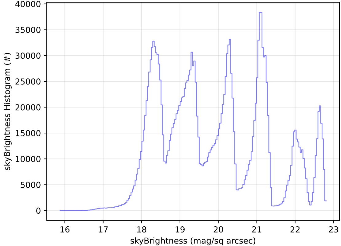
too_elab_2yr_r64_d3_ugrizy_v3.4_10yrs WFD all bands: skyBrightness Histogram
