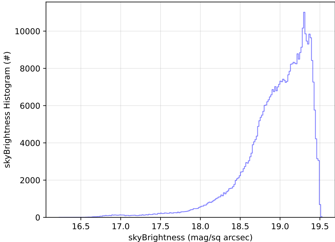
too_elab_2yr_r64_d3_ugrizy_v3.4_10yrs All sky z band: skyBrightness Histogram
