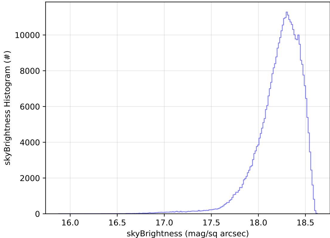
too_elab_2yr_r64_d3_ugrizy_v3.4_10yrs All sky y band: skyBrightness Histogram
