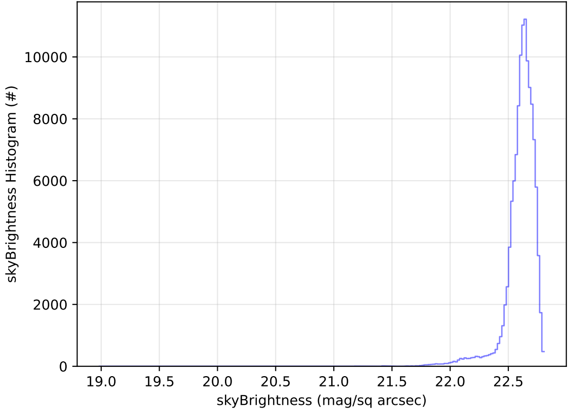
too_elab_2yr_r64_d3_ugrizy_v3.4_10yrs All sky u band: skyBrightness Histogram
