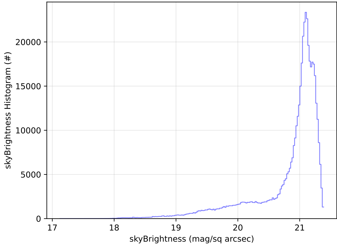
too_elab_2yr_r64_d3_ugrizy_v3.4_10yrs All sky r band: skyBrightness Histogram
