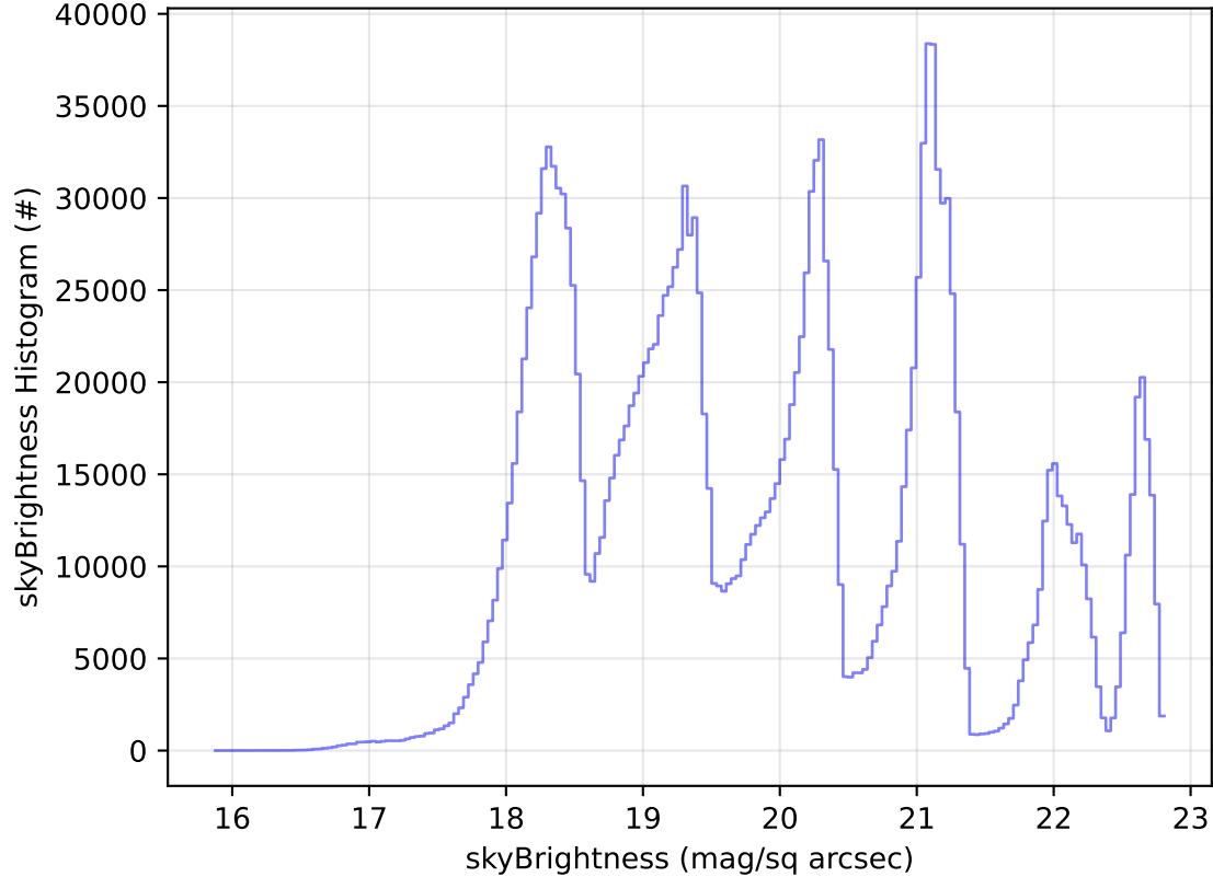
too_elab_2yr_r64_d3_ugrizy_v3.4_10yrs All sky all bands: skyBrightness Histogram
