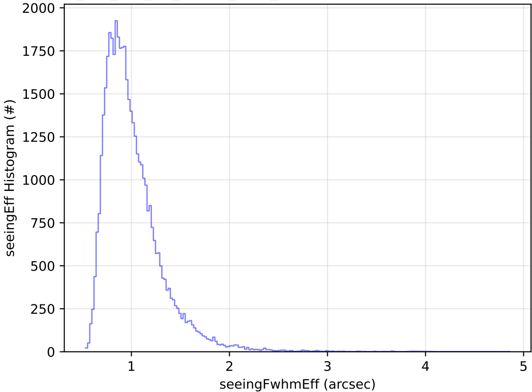
too_elab_2yr_r64_d3_ugrizy_v3.4_10yrs Yr 1 z band: seeingEff Histogram
