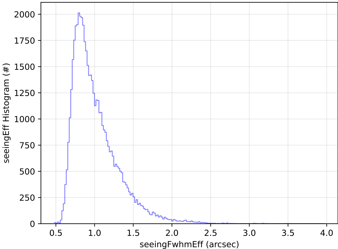
too_elab_2yr_r64_d3_ugrizy_v3.4_10yrs Yr 1 r band: seeingEff Histogram
