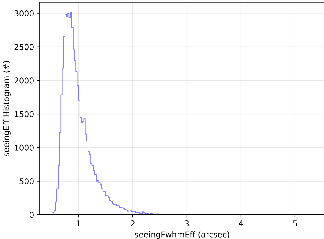
too_elab_2yr_r64_d3_ugrizy_v3.4_10yrs Yr 1 i band: seeingEff Histogram
