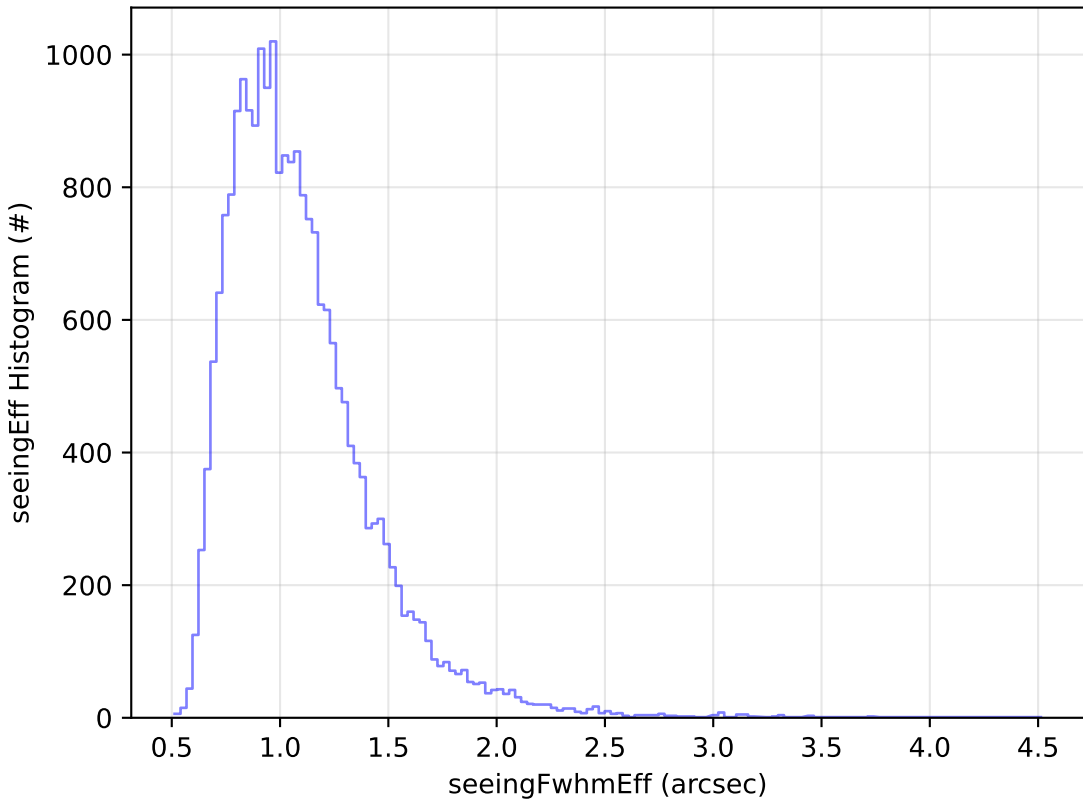
too_elab_2yr_r64_d3_ugrizy_v3.4_10yrs Yr 1 g band: seeingEff Histogram
