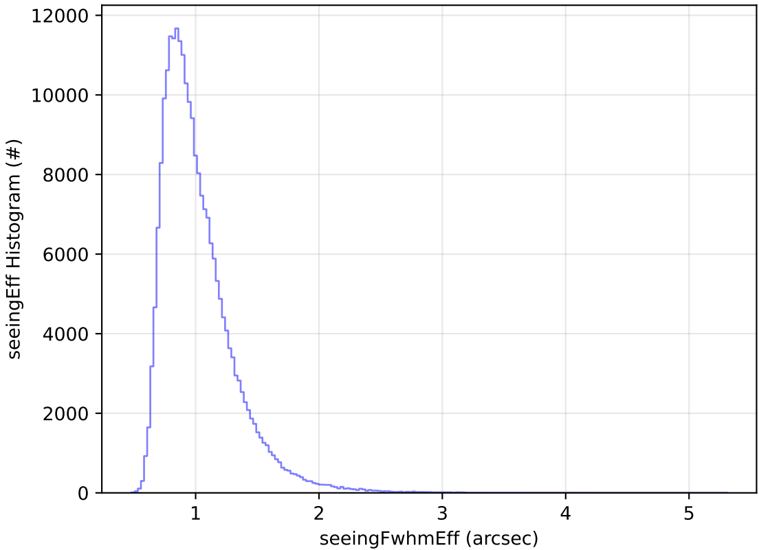
too_elab_2yr_r64_d3_ugrizy_v3.4_10yrs Yr 1 all bands: seeingEff Histogram
