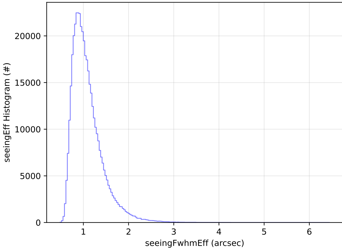
too_elab_2yr_r64_d3_ugrizy_v3.4_10yrs WFD z band: seeingEff Histogram
