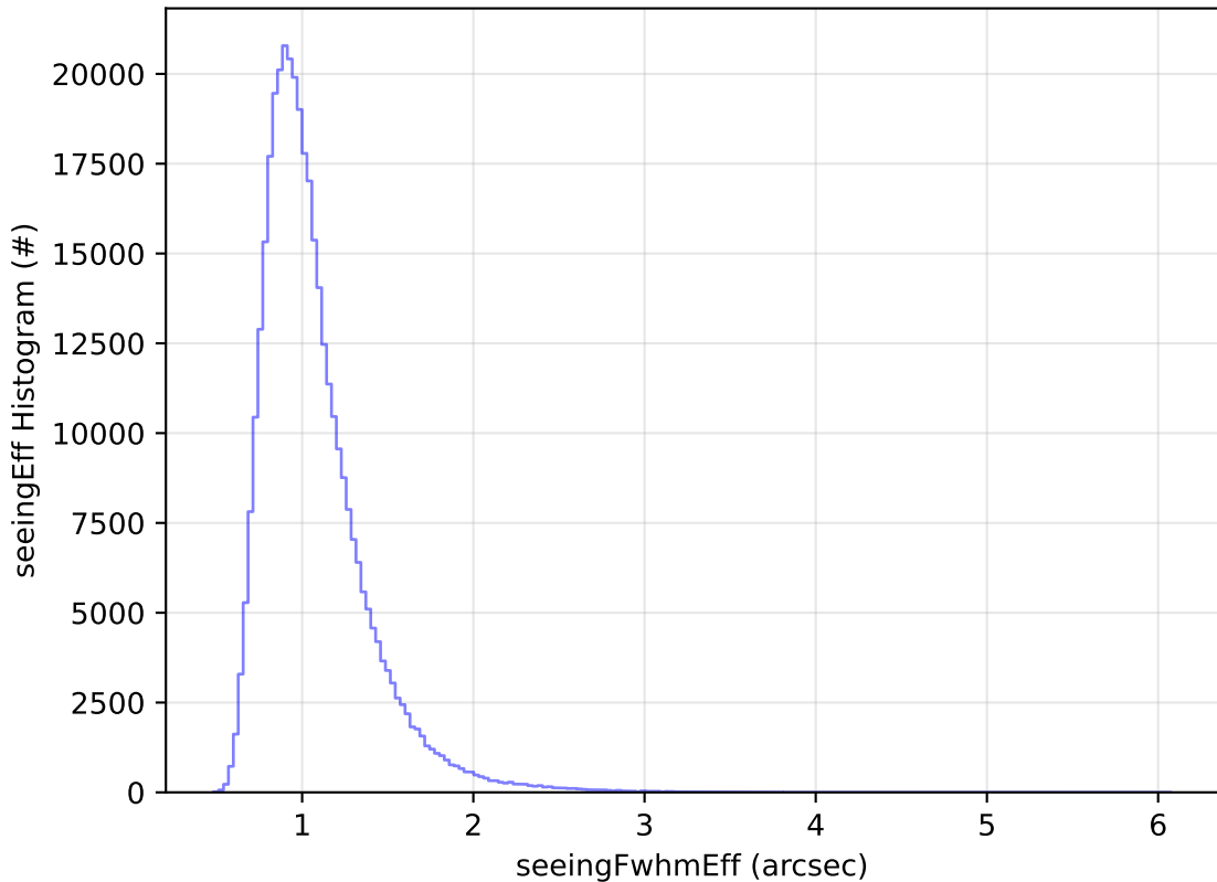
too_elab_2yr_r64_d3_ugrizy_v3.4_10yrs WFD y band: seeingEff Histogram
