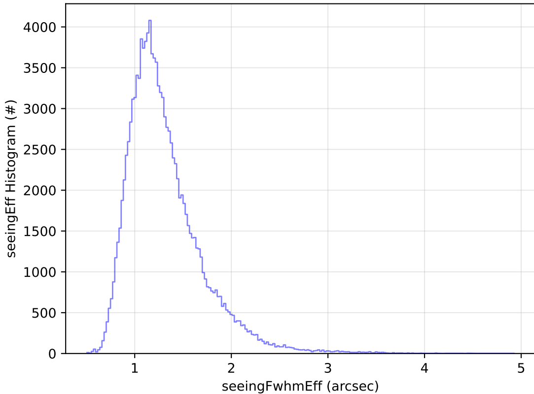
too_elab_2yr_r64_d3_ugrizy_v3.4_10yrs WFD u band: seeingEff Histogram
