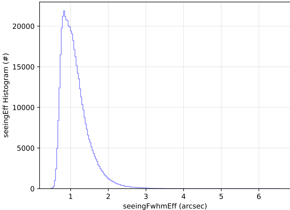
too_elab_2yr_r64_d3_ugrizy_v3.4_10yrs WFD r band: seeingEff Histogram
