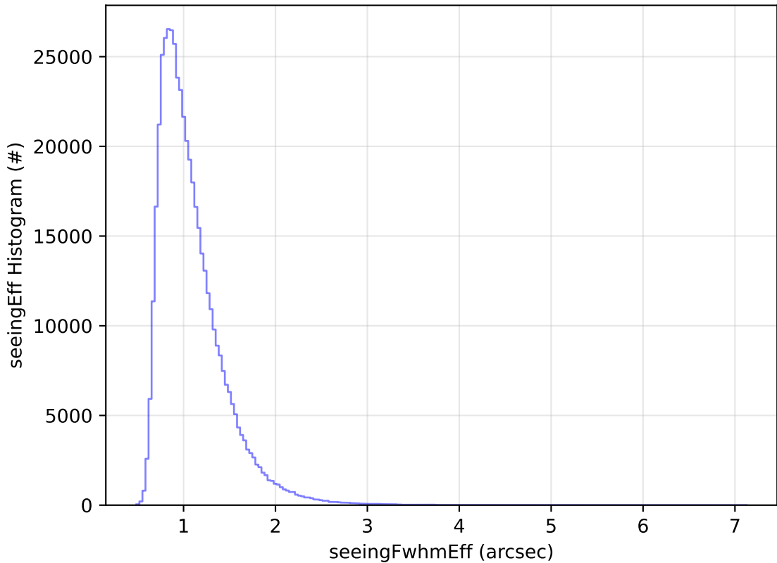
too_elab_2yr_r64_d3_ugrizy_v3.4_10yrs WFD i band: seeingEff Histogram
