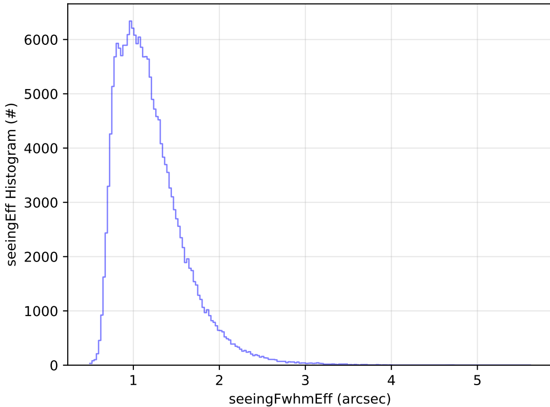
too_elab_2yr_r64_d3_ugrizy_v3.4_10yrs WFD g band: seeingEff Histogram
