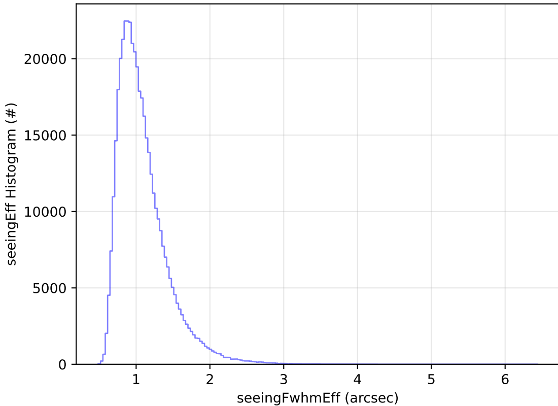
too_elab_2yr_r64_d3_ugrizy_v3.4_10yrs All sky z band: seeingEff Histogram
