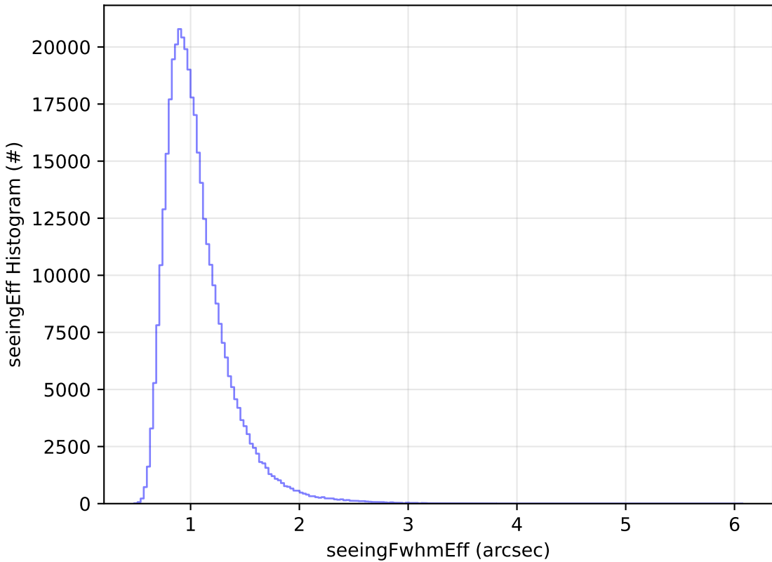
too_elab_2yr_r64_d3_ugrizy_v3.4_10yrs All sky y band: seeingEff Histogram
