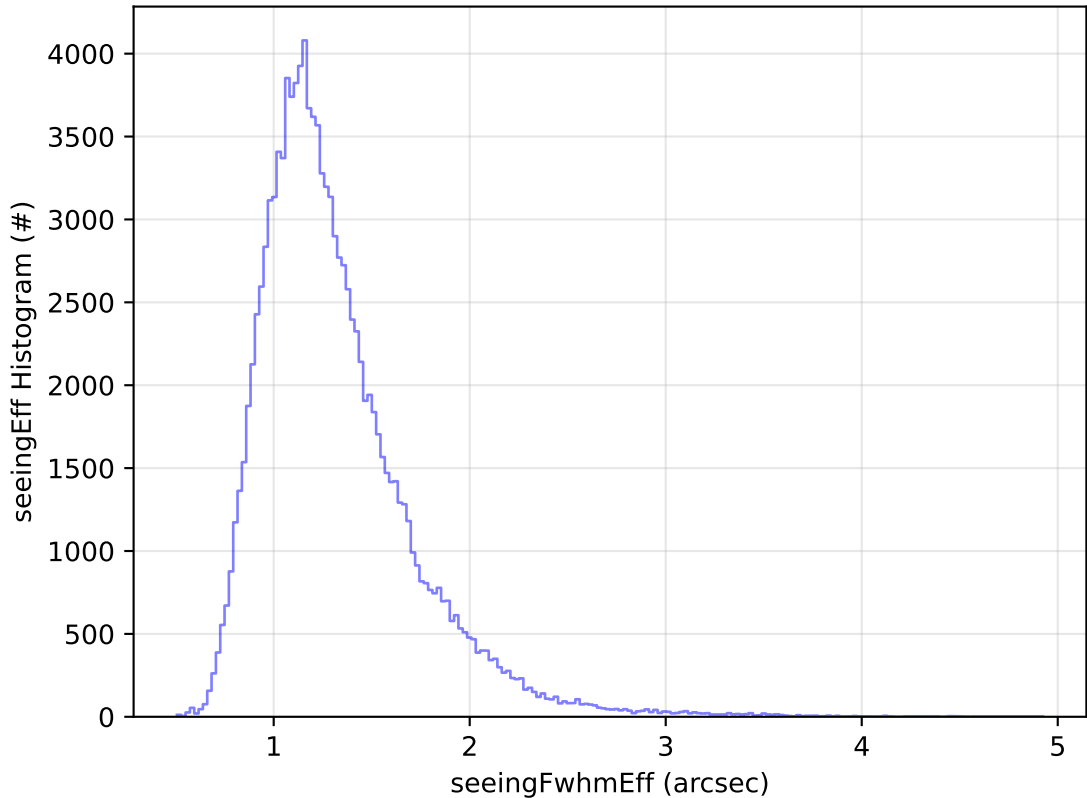
too_elab_2yr_r64_d3_ugrizy_v3.4_10yrs All sky u band: seeingEff Histogram
