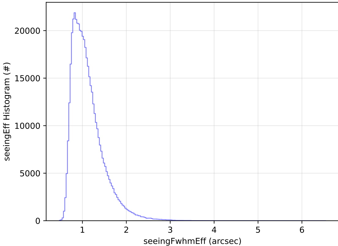
too_elab_2yr_r64_d3_ugrizy_v3.4_10yrs All sky r band: seeingEff Histogram
