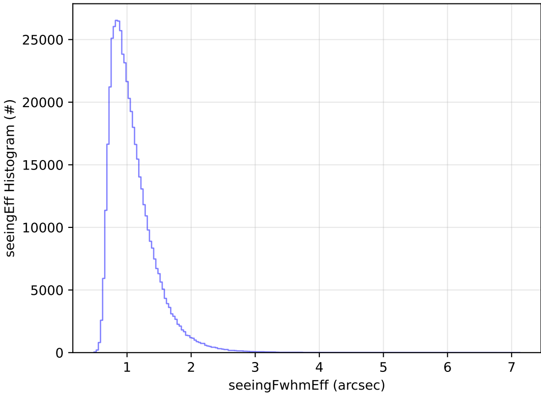
too_elab_2yr_r64_d3_ugrizy_v3.4_10yrs All sky i band: seeingEff Histogram
