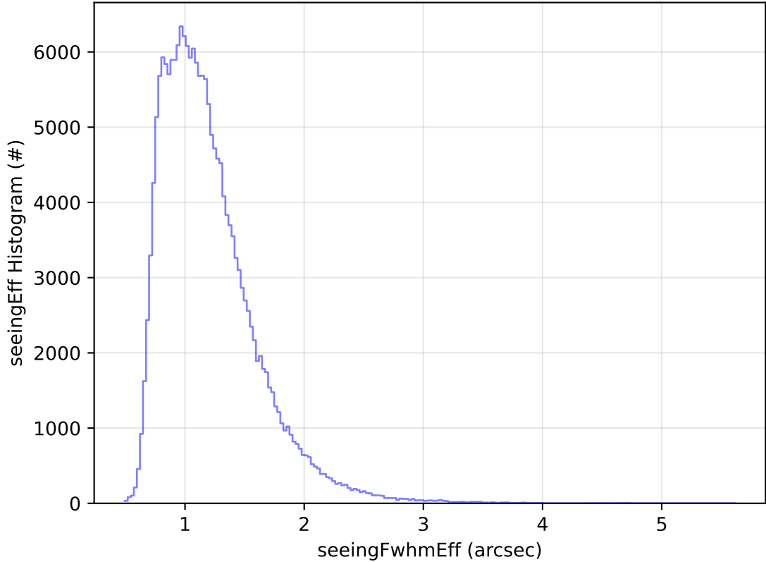
too_elab_2yr_r64_d3_ugrizy_v3.4_10yrs All sky g band: seeingEff Histogram
