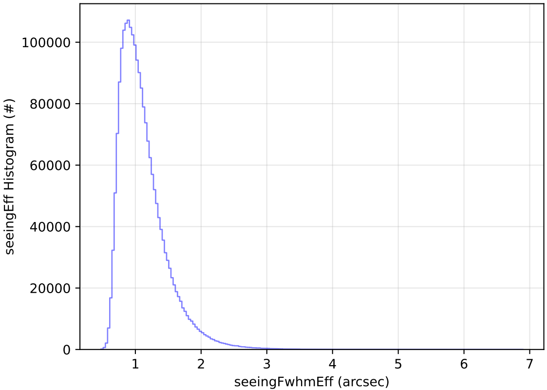
too_elab_2yr_r64_d3_ugrizy_v3.4_10yrs All sky all bands: seeingEff Histogram
