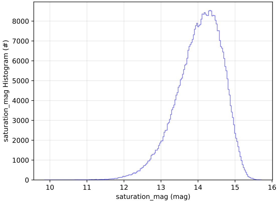
too_elab_2yr_r64_d3_ugrizy_v3.4_10yrs WFD z band: saturation_mag Histogram
