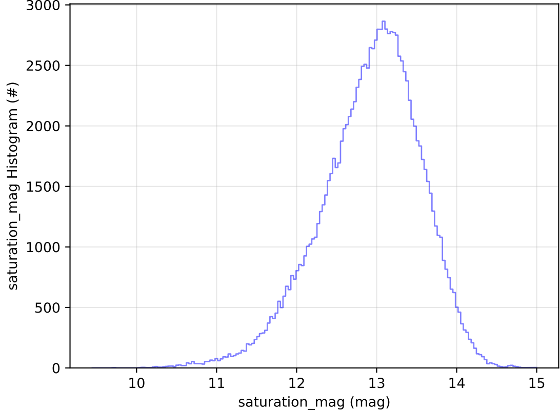
too_elab_2yr_r64_d3_ugrizy_v3.4_10yrs WFD u band: saturation_mag Histogram
