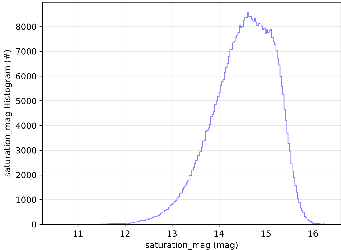
too_elab_2yr_r64_d3_ugrizy_v3.4_10yrs WFD r band: saturation_mag Histogram
