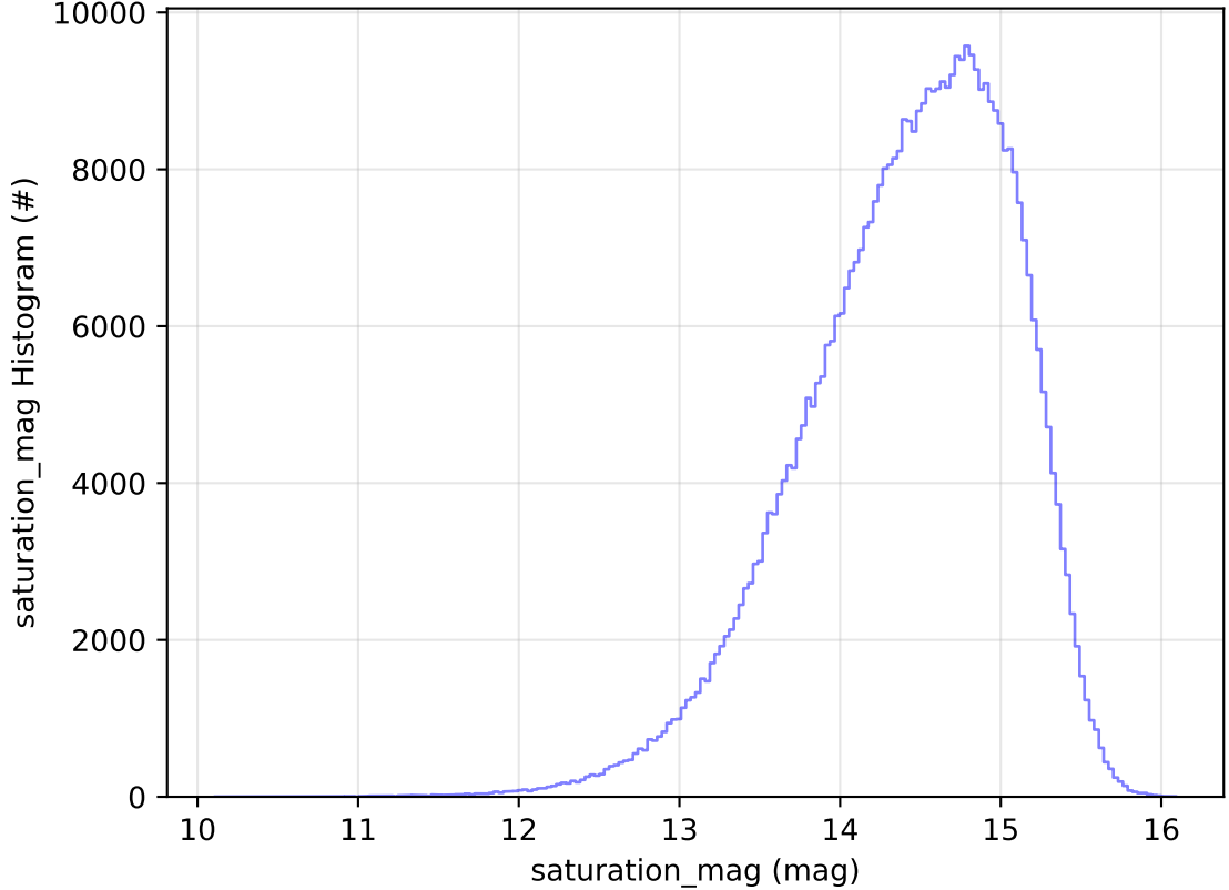
too_elab_2yr_r64_d3_ugrizy_v3.4_10yrs WFD i band: saturation_mag Histogram
