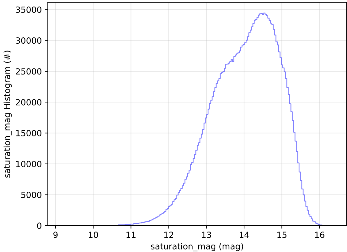
too_elab_2yr_r64_d3_ugrizy_v3.4_10yrs WFD all bands: saturation_mag Histogram
