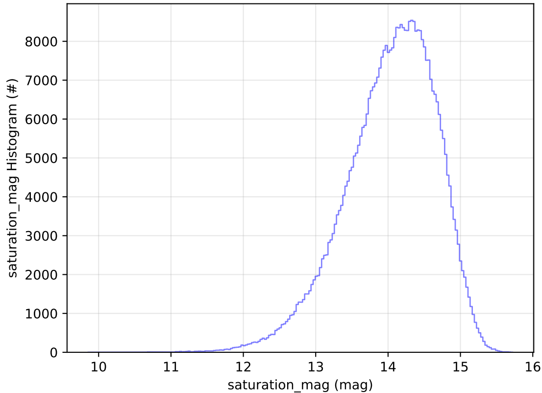
too_elab_2yr_r64_d3_ugrizy_v3.4_10yrs All sky z band: saturation_mag Histogram
