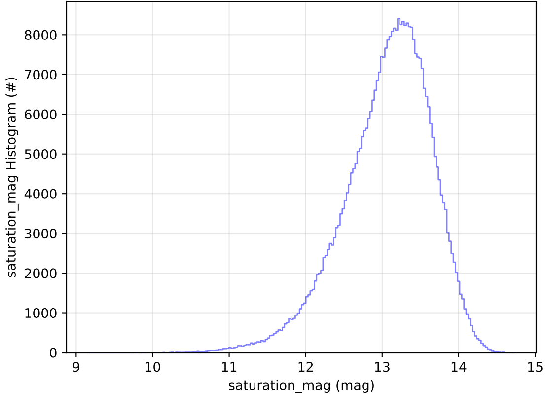
too_elab_2yr_r64_d3_ugrizy_v3.4_10yrs All sky y band: saturation_mag Histogram
