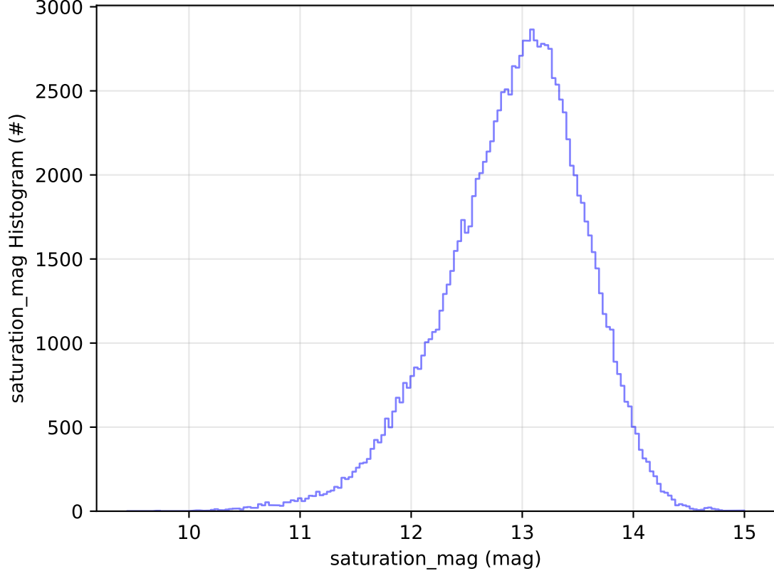
too_elab_2yr_r64_d3_ugrizy_v3.4_10yrs All sky u band: saturation_mag Histogram
