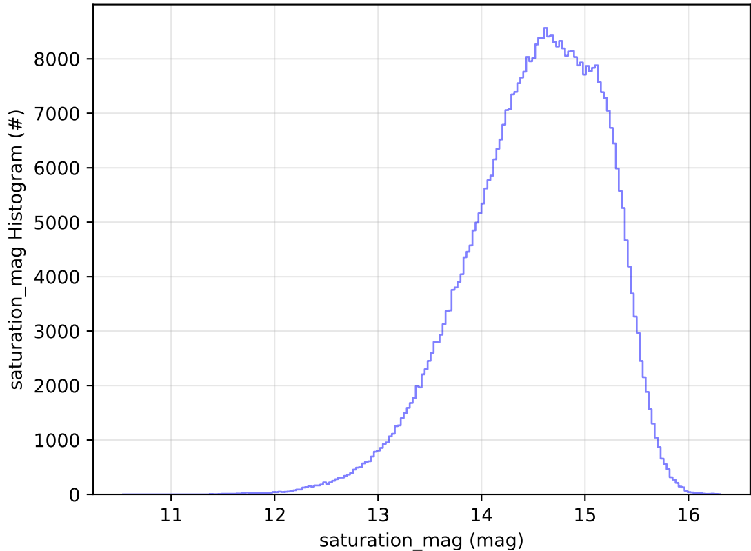
too_elab_2yr_r64_d3_ugrizy_v3.4_10yrs All sky r band: saturation_mag Histogram
