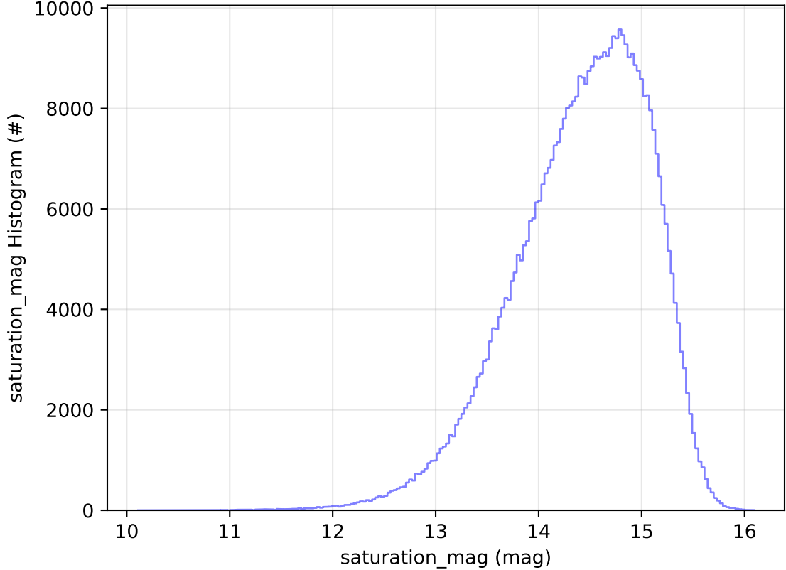
too_elab_2yr_r64_d3_ugrizy_v3.4_10yrs All sky i band: saturation_mag Histogram
